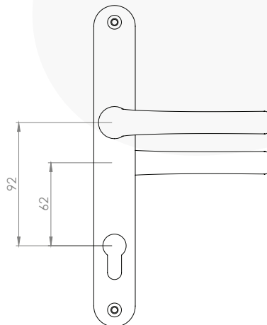
OFFSET LEVER AVAILABLE ON INTERMEDIATE AND LONG BACKPLATE ONLY
