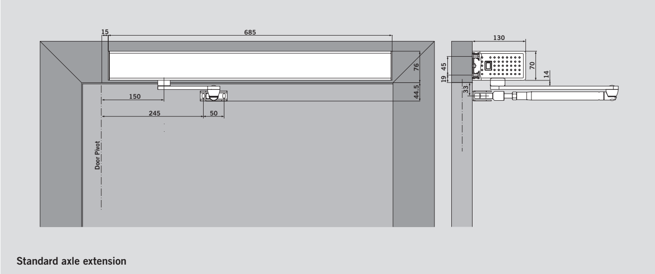
View: BASIC cover, push-version, pivoted door
