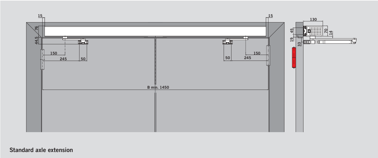
View: CONTINUOUS cover, push-version
