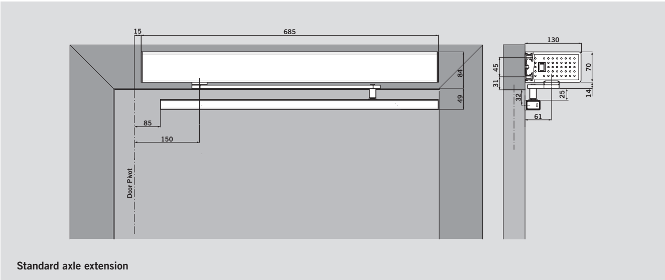
View: BASIC cover, pull-version, 25 mm drive arm pin, pivoted door
