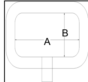
Hoop Dimensions Dia A = 320mm Dia B = 160mm
