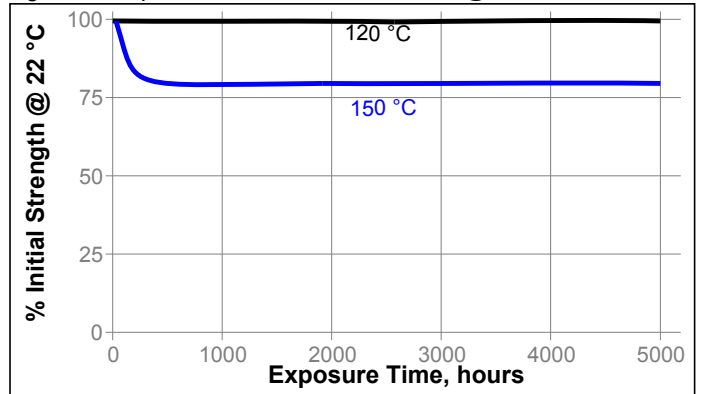
Chemical/Solvent Resistance Aged under conditions indicated and tested @ 22 °C
