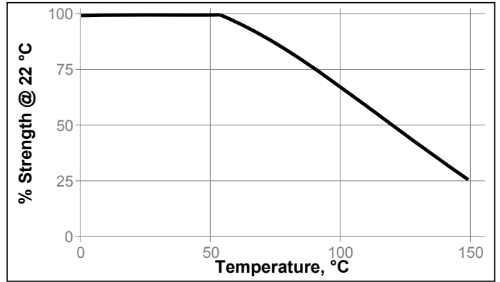
Heat Aging Aged at temperature indicated and tested @ 22 °C
