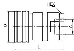
Female Thread
