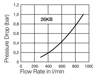
Flow Diagram (Water)
