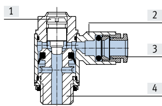
One-way flow control valve
