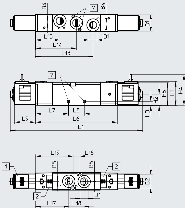
[1] Solenoid coil interface type C [2] Space for inscription label [7] For screw M3
