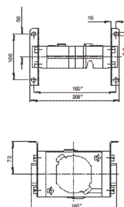
Bracket mounting (R68G)
