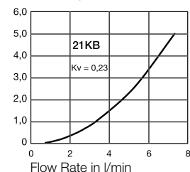
Flow Diagram (Water)
