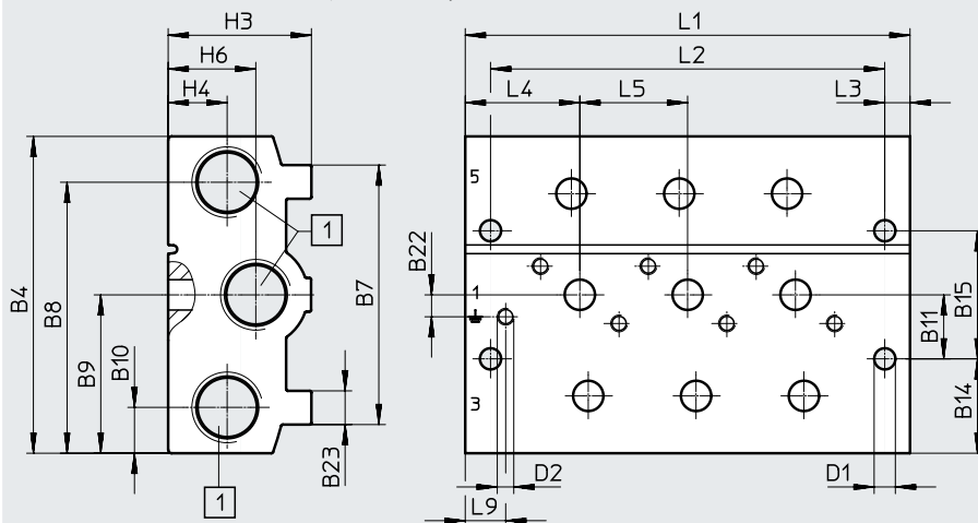
[1] Ports 1, 3 and 5: G1/2
