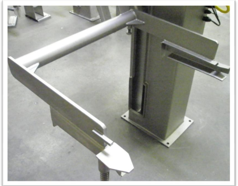
Tapered Loading Track and spring-loaded cart lock
