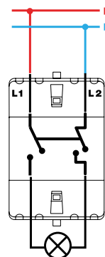
Interruptor bipolar / Double pole switch XXXX133-XXX
