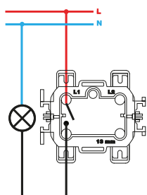
Interruptor unipolar / Single-pole switch 73101-39
