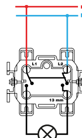
Interruptor bipolar / Double pole switch 73131-39
