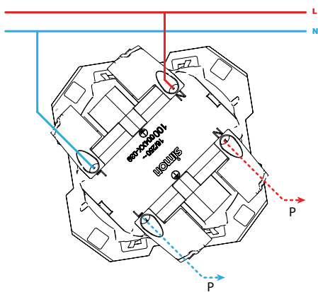
Base bipolar / Two-pole 10000431-039
