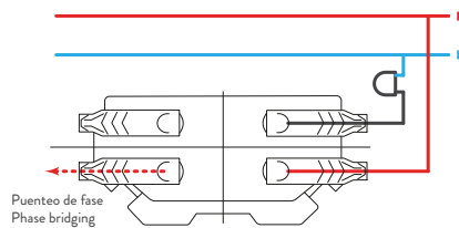
Pulsador / Push button switch 10000150-039
