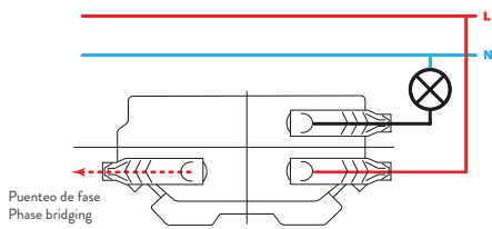
Interruptor unipolar / Single-pole switch 10000101-039
