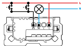
Luz - Interruptor regulable IO / 2-wire PC dimmer switch 1000320-039
