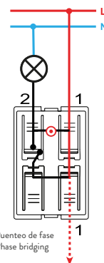
Pulsador con luminoso / Push button switch with light 7700160-039
