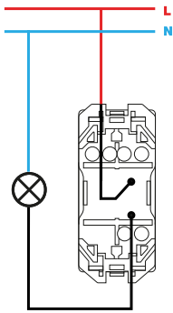
Interruptor unipolar / Single-pole switch 20000101-XXX
