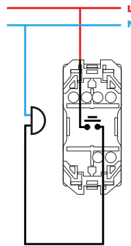
Pulsador neutro / Neutral push button switch 2000015X-XXX
