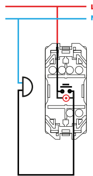
Pulsador neutro luminoso / Neutral push button switch with light indicator 2000016X-XXX
