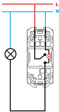
Interrupor piloto / Pilot switch 20000102-XXX
