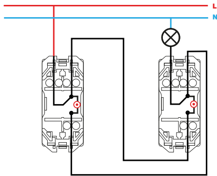
Conmutador luminoso / 2-way switch with light indicator 20000204-XXX
