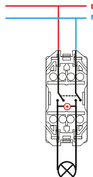
Interrupor bipolar piloto / Double pole pilot switch 20000134-XXX
