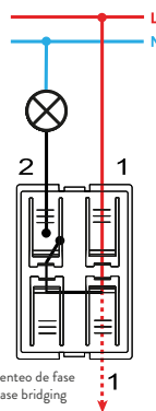
Interruptor unipolar / Single-pole switch 7700101-039
