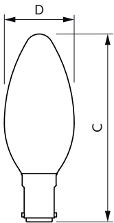
MAS LEDCandleDT3.4-40W B15 927 B35CL G
