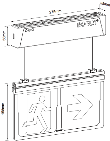
Dimension Diagram
