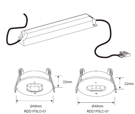
Dimension Diagram
