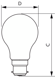
MAS LEDBulbDT10.5-100W B22 927A60CLG
