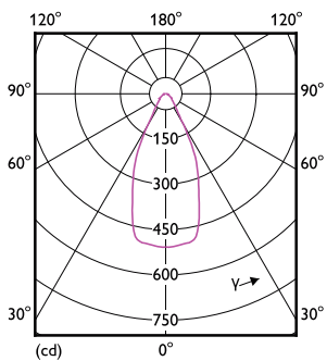
LEDspots MAS SLR 20W AR111 G53 927 45D-LDD LDD
