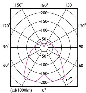
Light Distribution Diagram - MAS LEDcandle DT 5.5-40W E27 B38 CL UK
