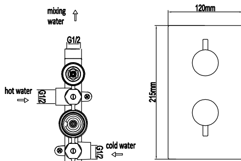
Single outlet thermostatic valve
