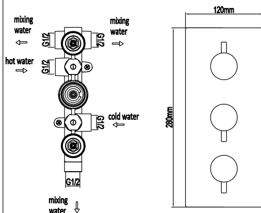
Triple outlet thermostatic valve
