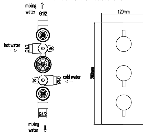
Double outlet thermostatic valve
