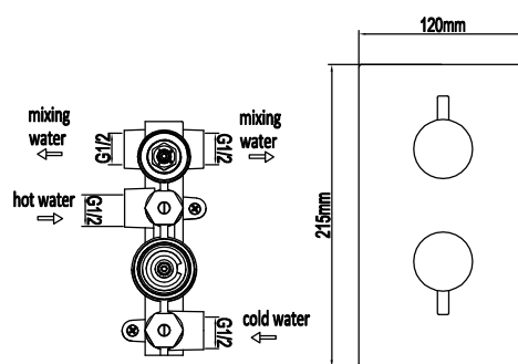
Double outlet thermostatic valve
