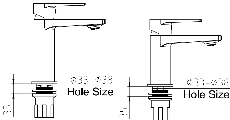
Tall Basin Mono taps
