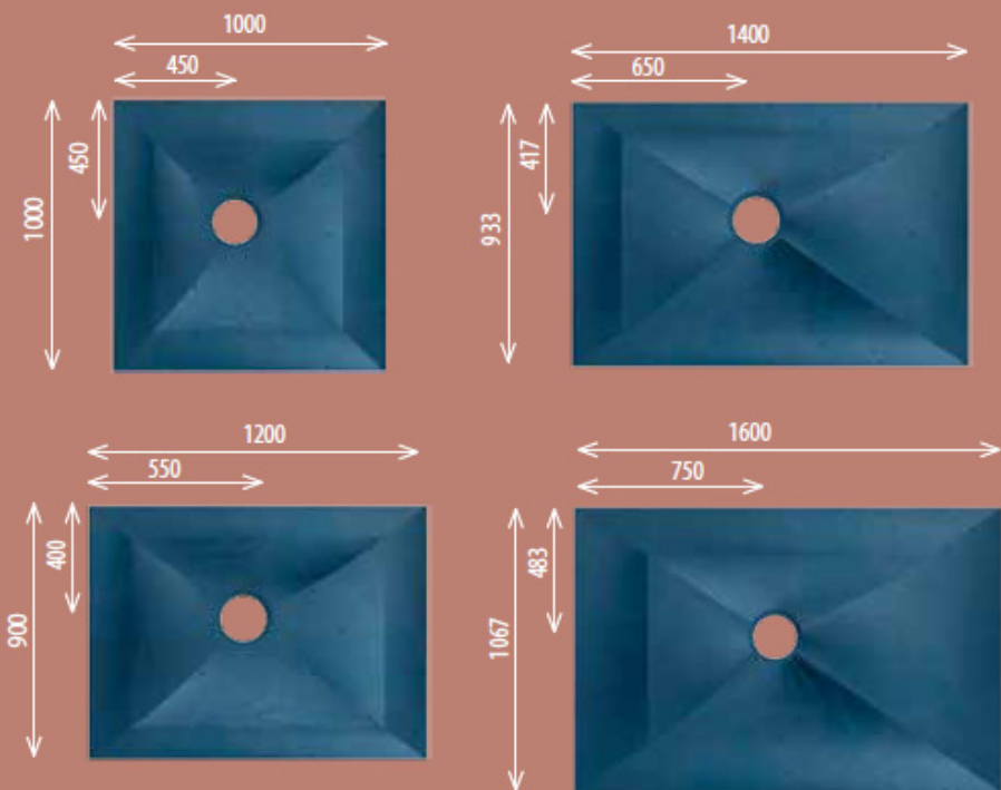
Floor Formers
