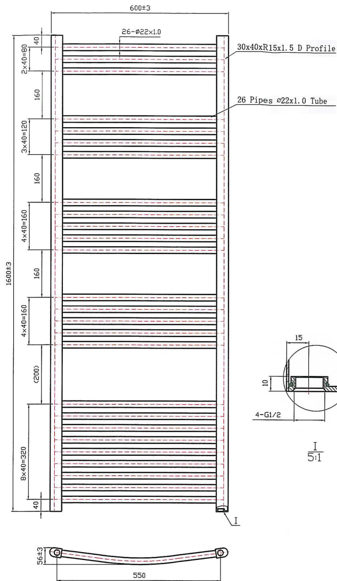
1600*600 26 pipes Curved
