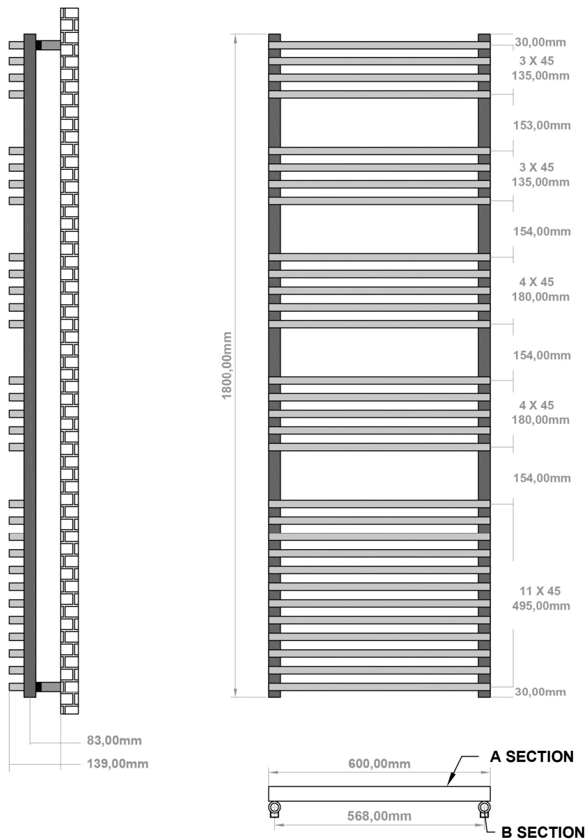
A SECTION
