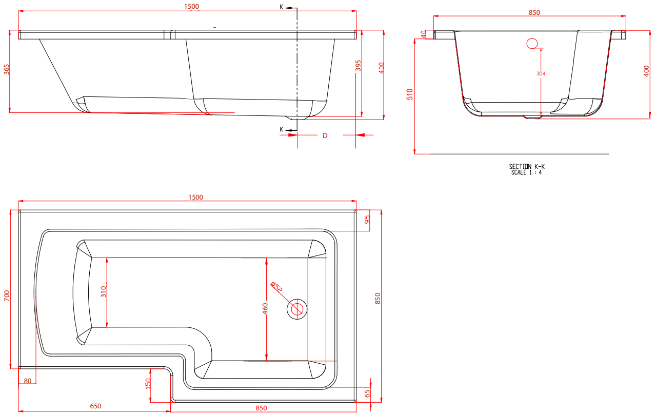
Shannon L Shaped RH 1500 x 850 x 400
