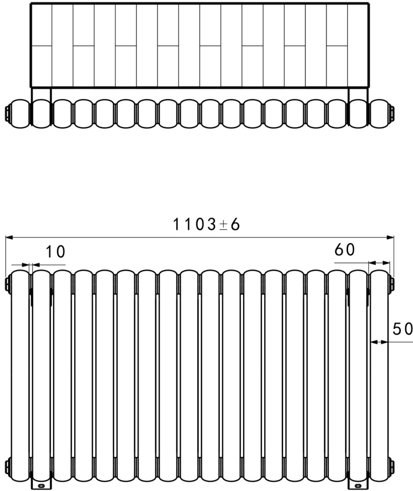
Top view
