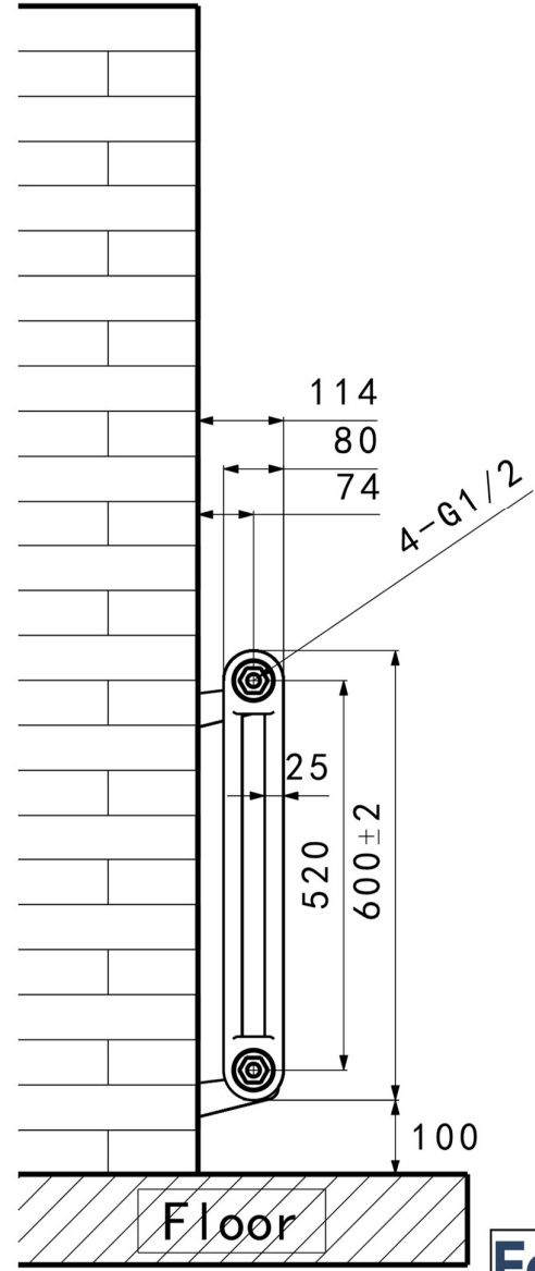
Side view
