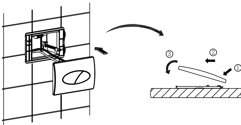
(5) Fix the control plate as shown in the picture
