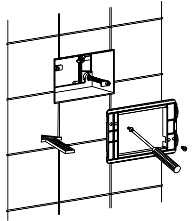
(3) Fix the control plate base
