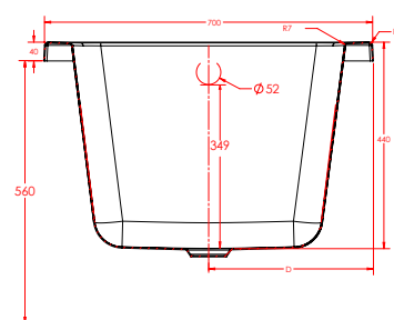
SECTION C-C SCALE 1 : 4
