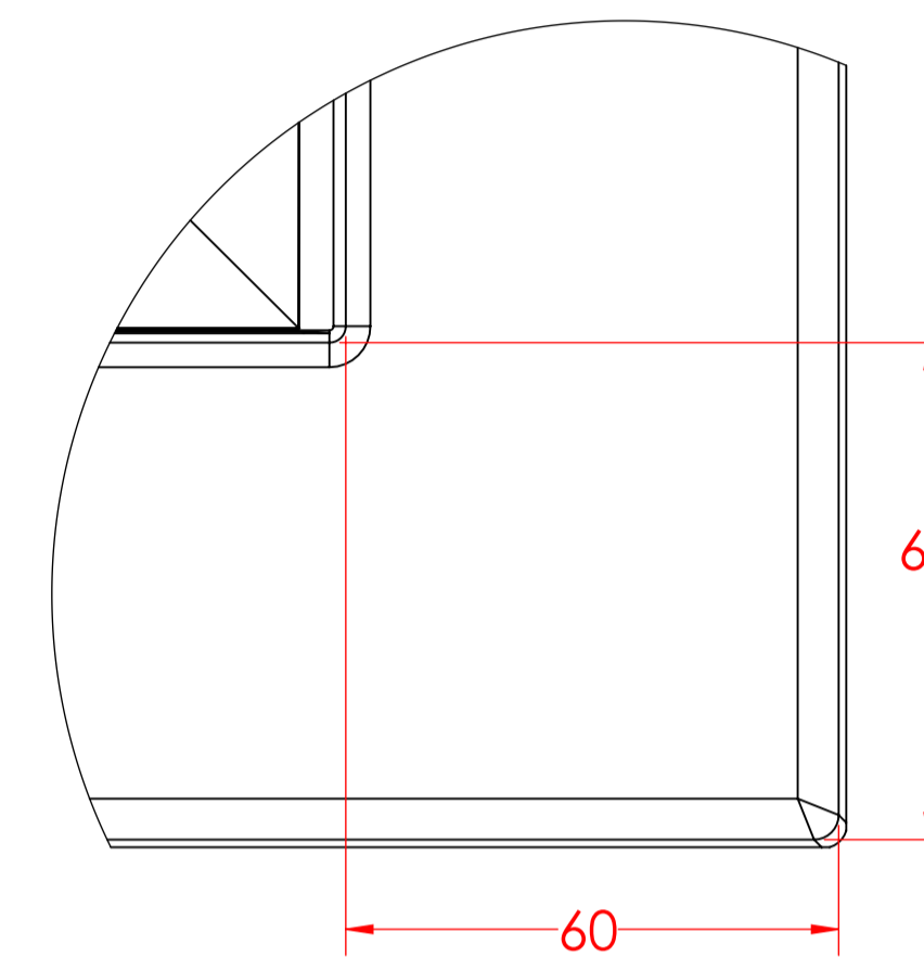
DETAIL D SCALE 1 : 1
