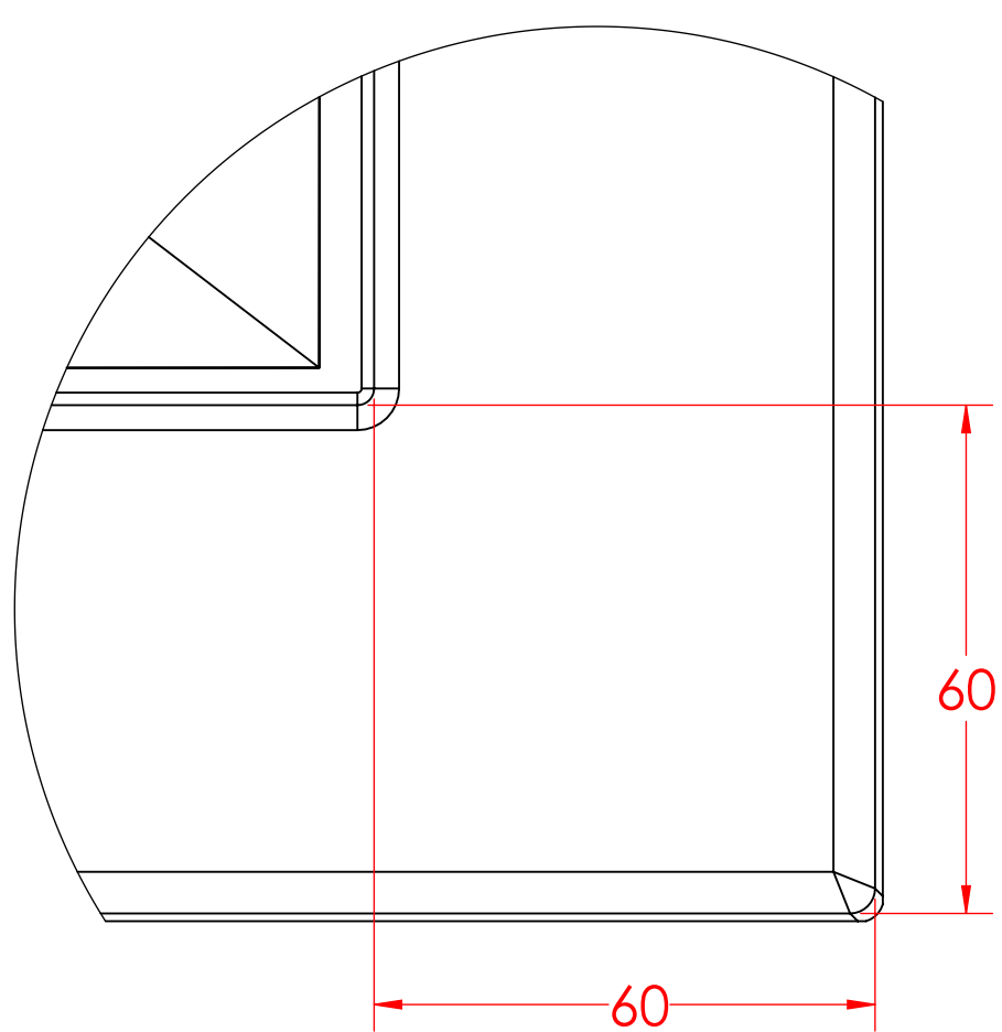
DETAIL D SCALE 1 : 1
