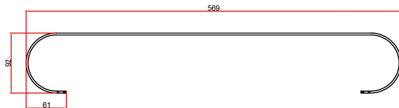
Sandhurst Vertical 485mm Width Towel Hanger :
