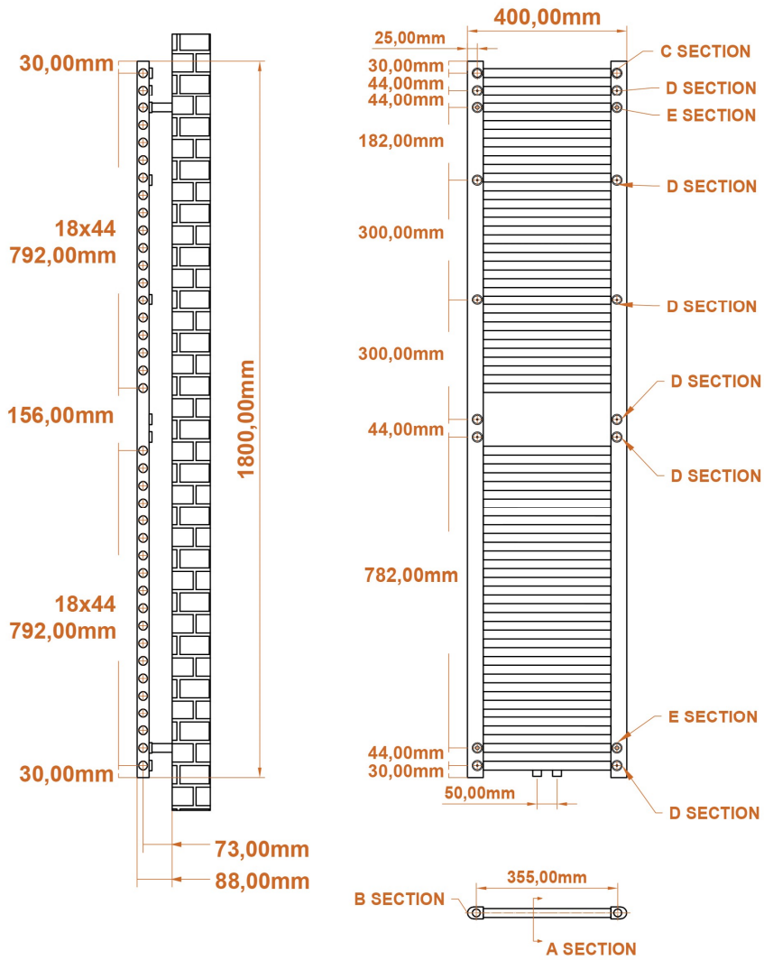
A SECTION
