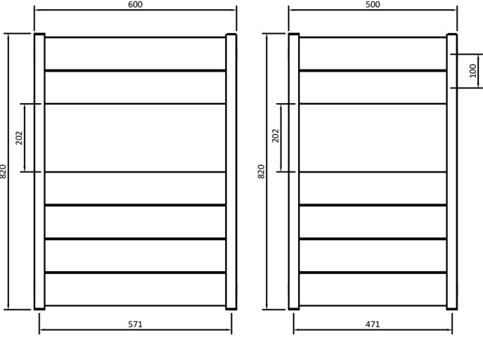
6 rails 2+4
