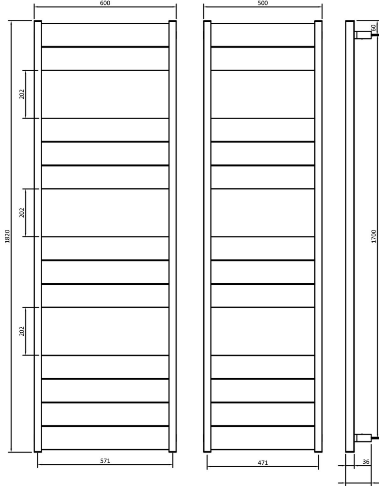
12 rails 2+3+3+4
