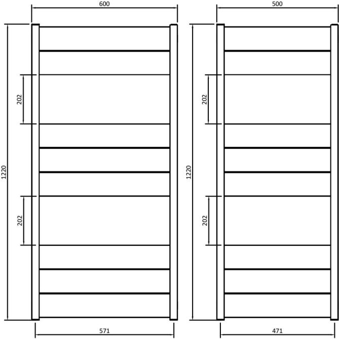
8 rails 2+3+3
