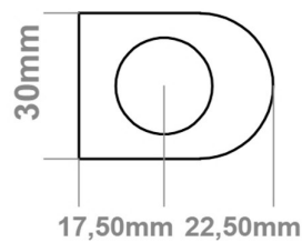
B SECTION
