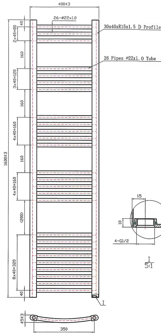
1600*400 26 pipes Curved
