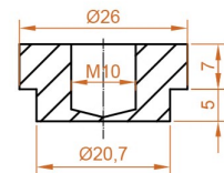
E SECTION
