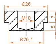
E SECTION
