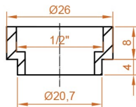
C SECTION
