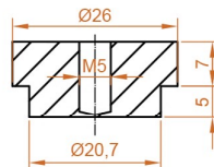
D SECTION
