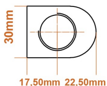
B SECTION
