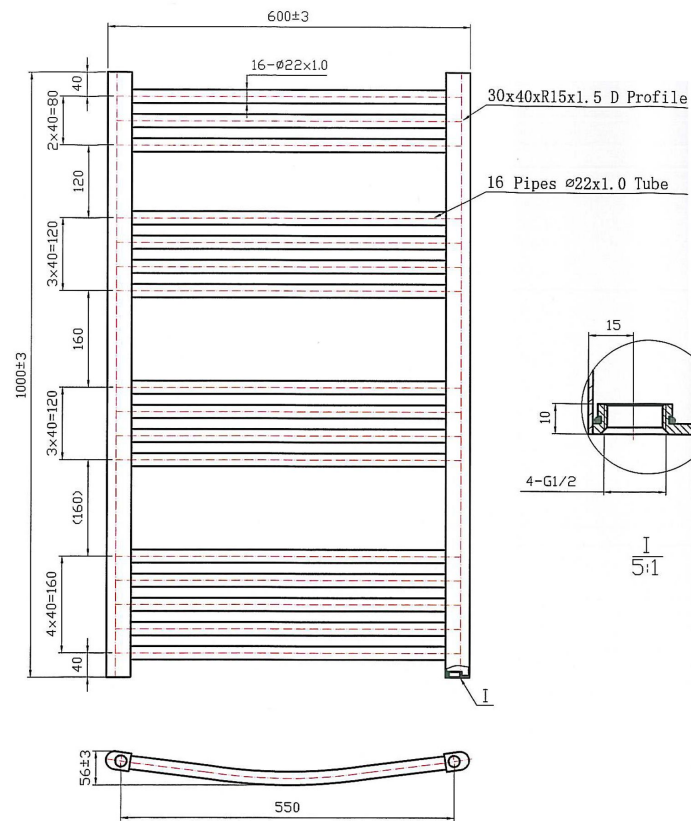
1000*600 16 pipes Curved
