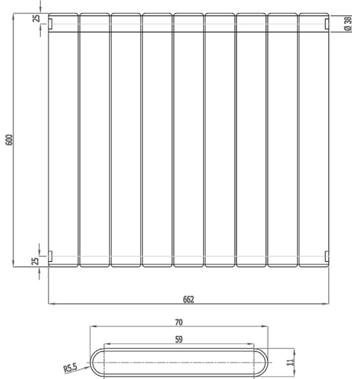
Vertical Installation
