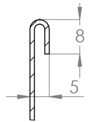
DETAIL Q SCALE 1 : 1
