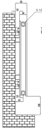
Horizontal Installation
