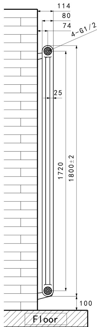
Side view
