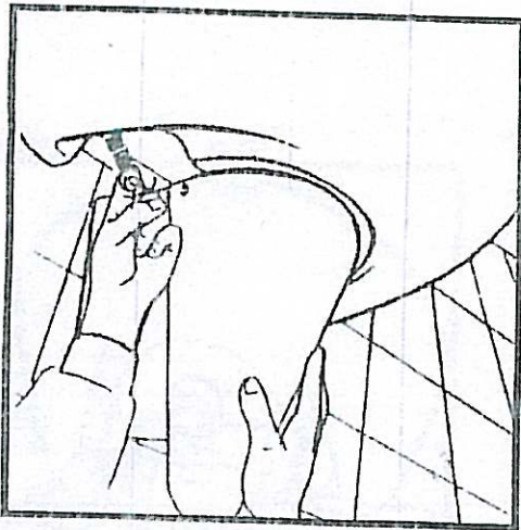
6) Take the spring from the outside of the trapez-cover If the trapez-cover is too loose then put the spring on the next hole of the mounting elements
