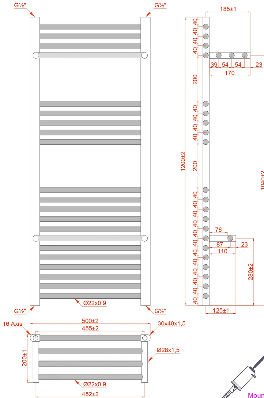
Haddenham Technical Drawing ( 61.0068 - 61.0070 - 61.0072 )
