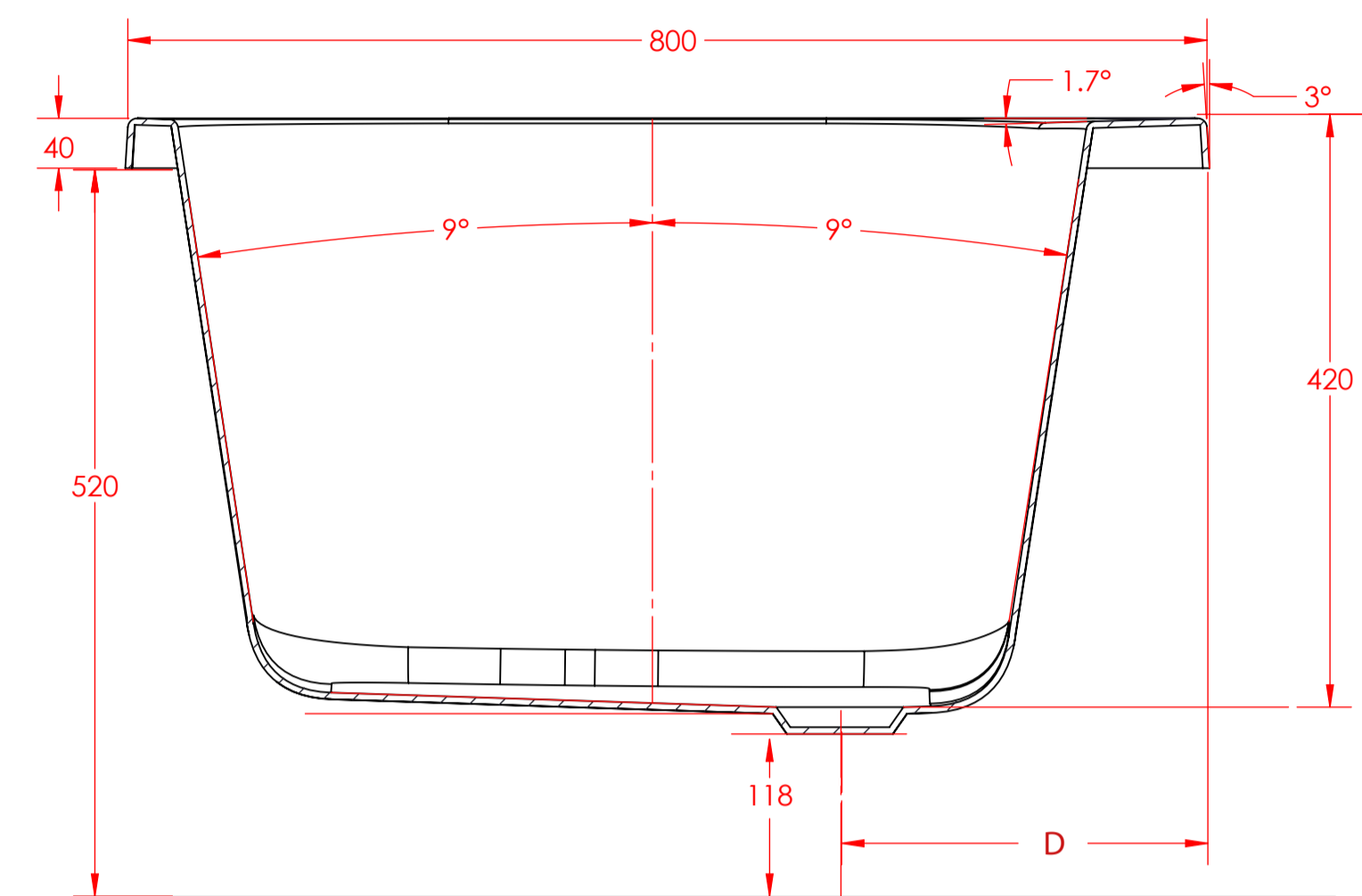
SECTION E-E SCALE 1 : 5
